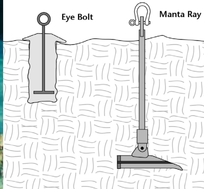
Figure 10: fixed eco-mooring two pictures left eye bolt and right manta ray (padi, 1996; reef relief founders)
